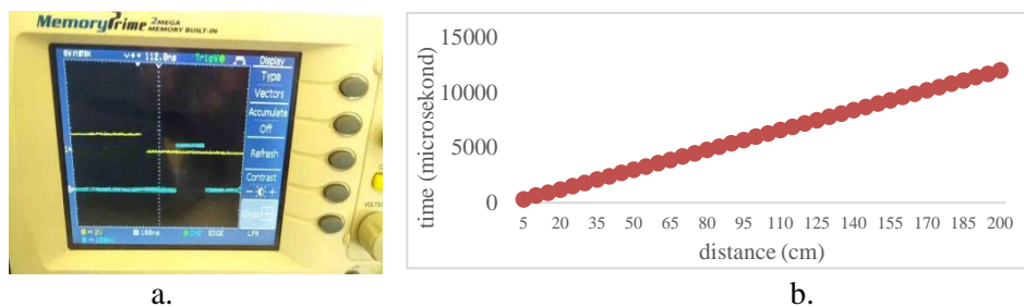
Figure 12 a. Output of sensor ultrasonic, b. Relation of time width and the distance
