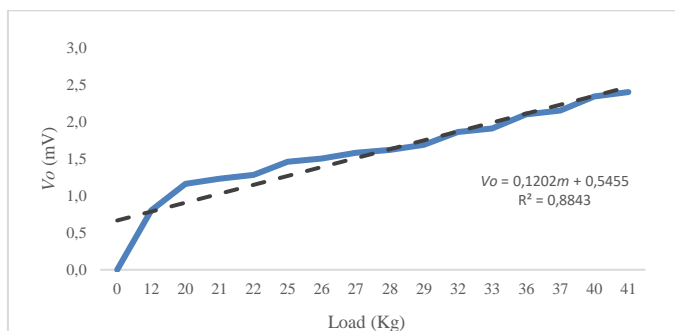
Figure 13. Relation of output voltage and the mass
