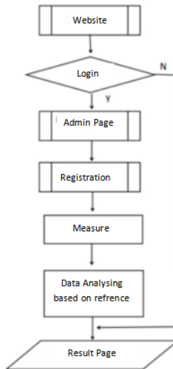
Figure 4. Flowchart of the website page
